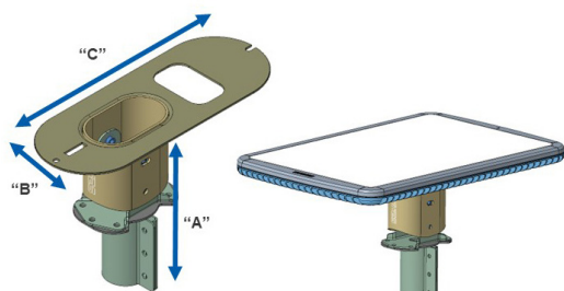
(1) Mast Adapter Mount
