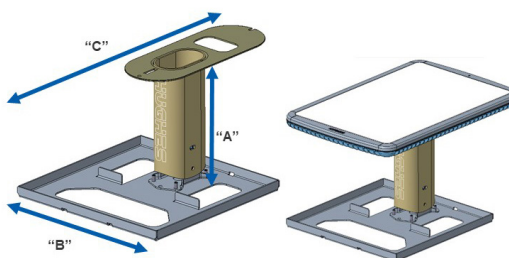
(2) Non-Penetrating Mount with Tall Stanchion
